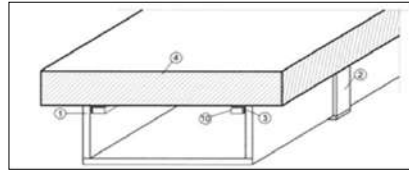
3-sided duct
